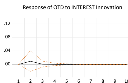
Response to Cholesky One S.D. (d.f. adjusted) Innovations \pm 2 Monte Carlo S.E.s
