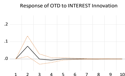
Response to Cholesky One S.D. (d.f. adjusted) Innovations \pm 2 Monte Carlo S.E.s
