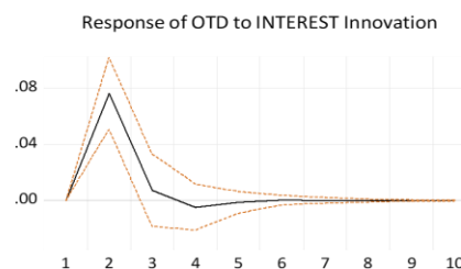
Response to Cholesky One S.D. (d.f. adjusted) Innovations ± 2 Monte Carlo S.E.s
