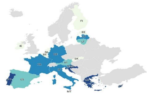
univariate clustering MINMAX
